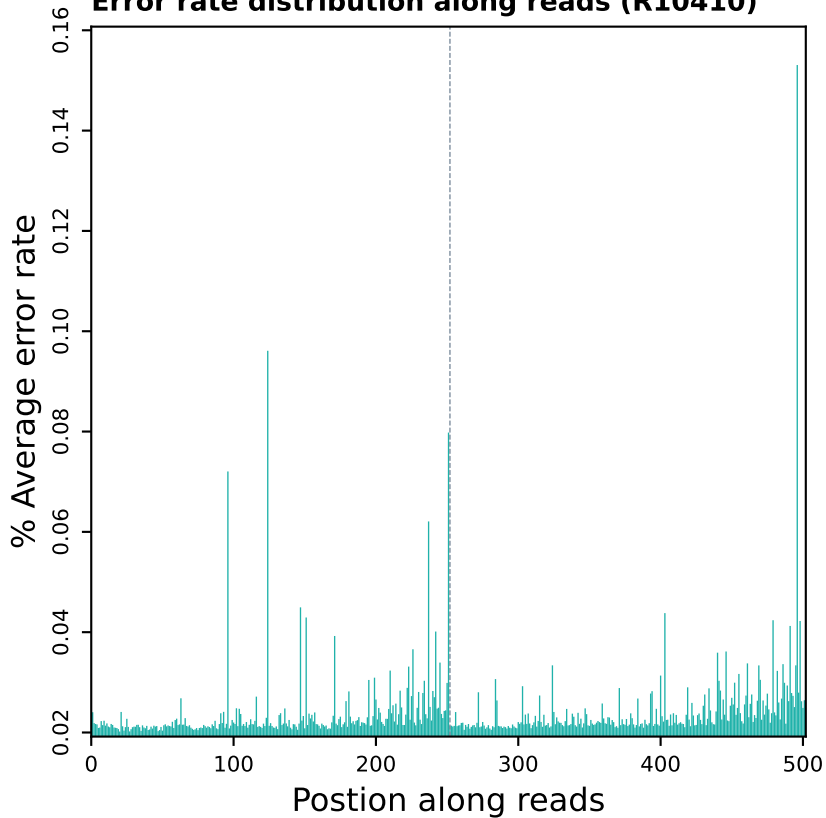
Error rate distribution along reads (R10410)
